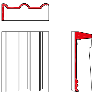
chaperongevelpan links 90°
